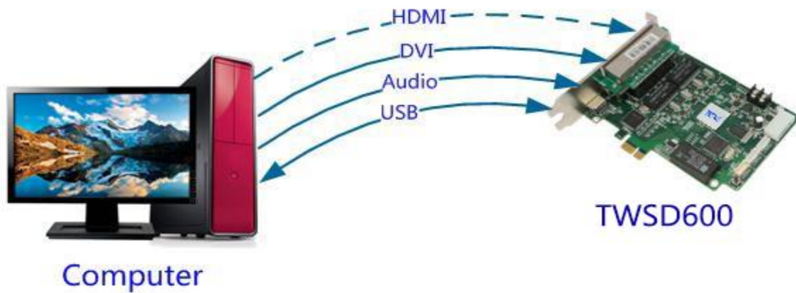
Fig. 2 Connection diagram
